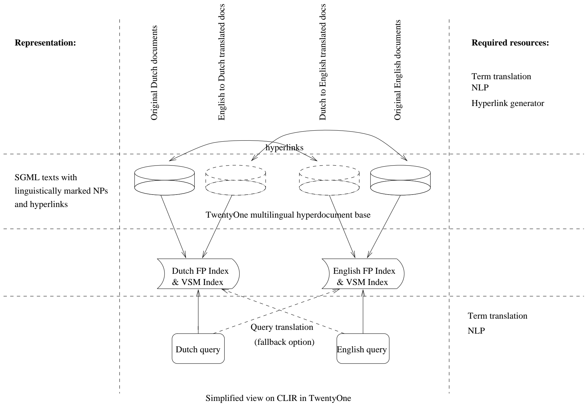
Figure 1: Overview of CLIR in TwentyOne
